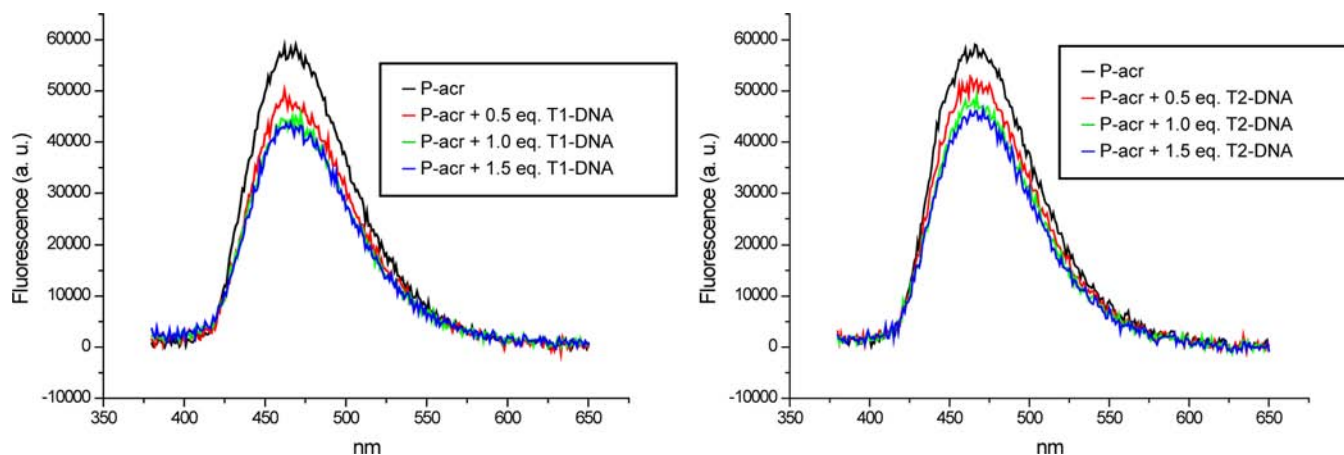
Figure 2. Emitted fluorescence of P-acr alone (black lines) and after addition of 0.5 (red line), 1 (green line), and 1.5 eq (blue line) of T1-DNA (left panel) or T2-DNA (right panel). The mixtures were irradiated at 370 nm with a cutoff at 375 nm and a temperature of 24 °C.
