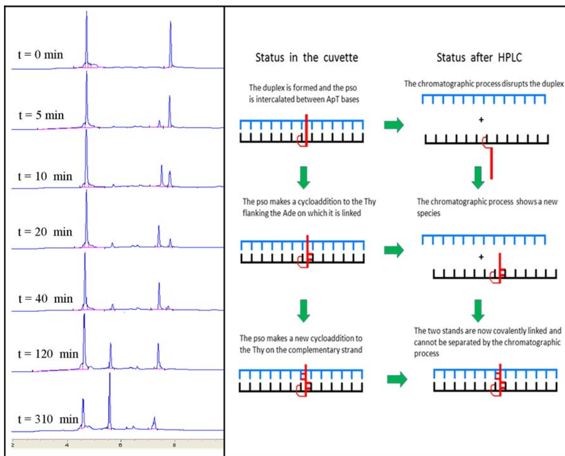
Figure 1. Left panel: HPLC chromatograms of samples taken from the mixture P-so with T1-DNA upon irradiation at 350 nm, at the indicated times. Right panel: a cartoon with our explanation of the underlying events.
